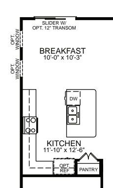
OPT. KITCHEN ISLAND
