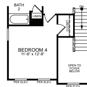
OPT. BEDROOM 4 WITH OPEN FOYER
