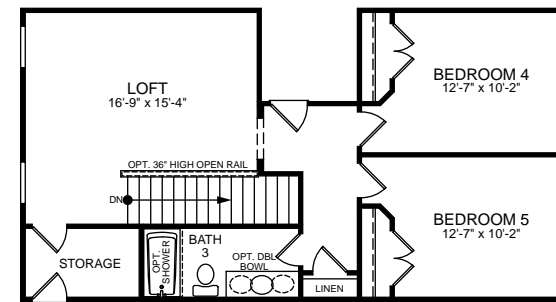
OPT. SECOND FLOOR W/ BEDROOM 4 & BEDROOM 5
