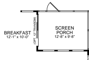
OPT. SCREEN PORCH
