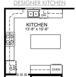
OPT. ALTERNATE DESIGNER KITCHEN
