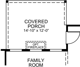
OPT. COVERED PORCH
