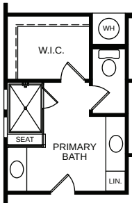
OPT. LUXURY SHOWER AT PRIMARY BATH
