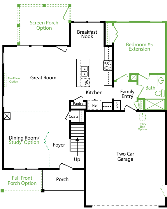
FIRST FLOOR | SCREEN PORCH, BEDROOM #5 EXTENSION WITH FULL BATH
